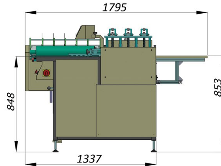
Above: GC-760 XL PRO Dimensions (Side View)
